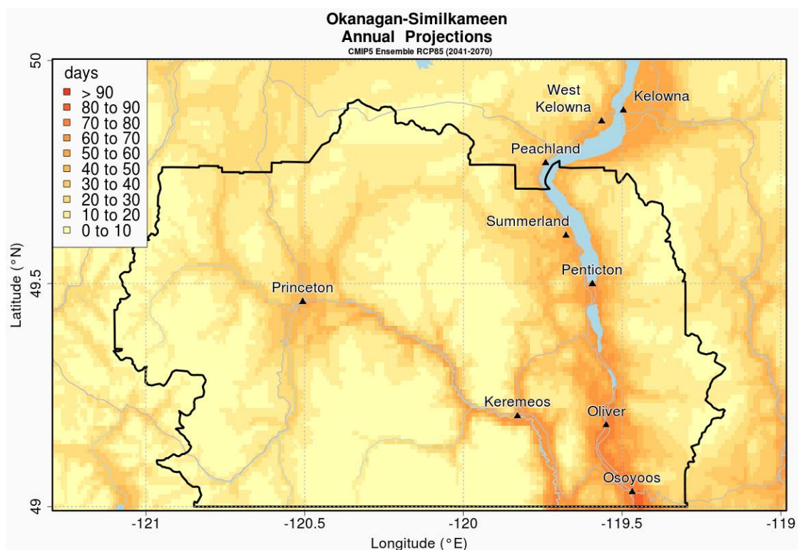
FIGURE A2-4 (RDOS): DAYS ABOVE 30°C – FUTURE (2050s)
